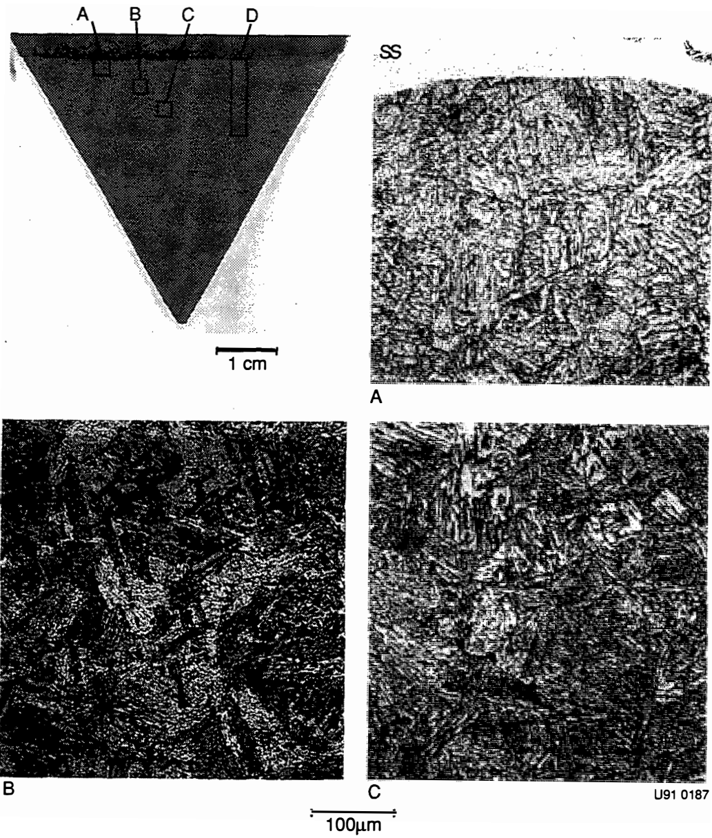
Sample E-8 (m-3)
